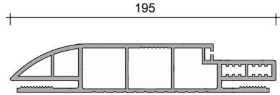
195 mm OVAL KASA 195 mm OVAL FRAME
