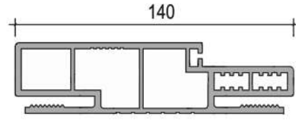
140 mm KASA 140 mm FRAME
