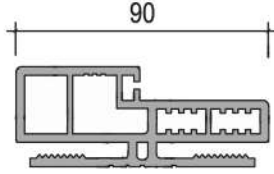
90 mm KASA 90 mm FRAME
